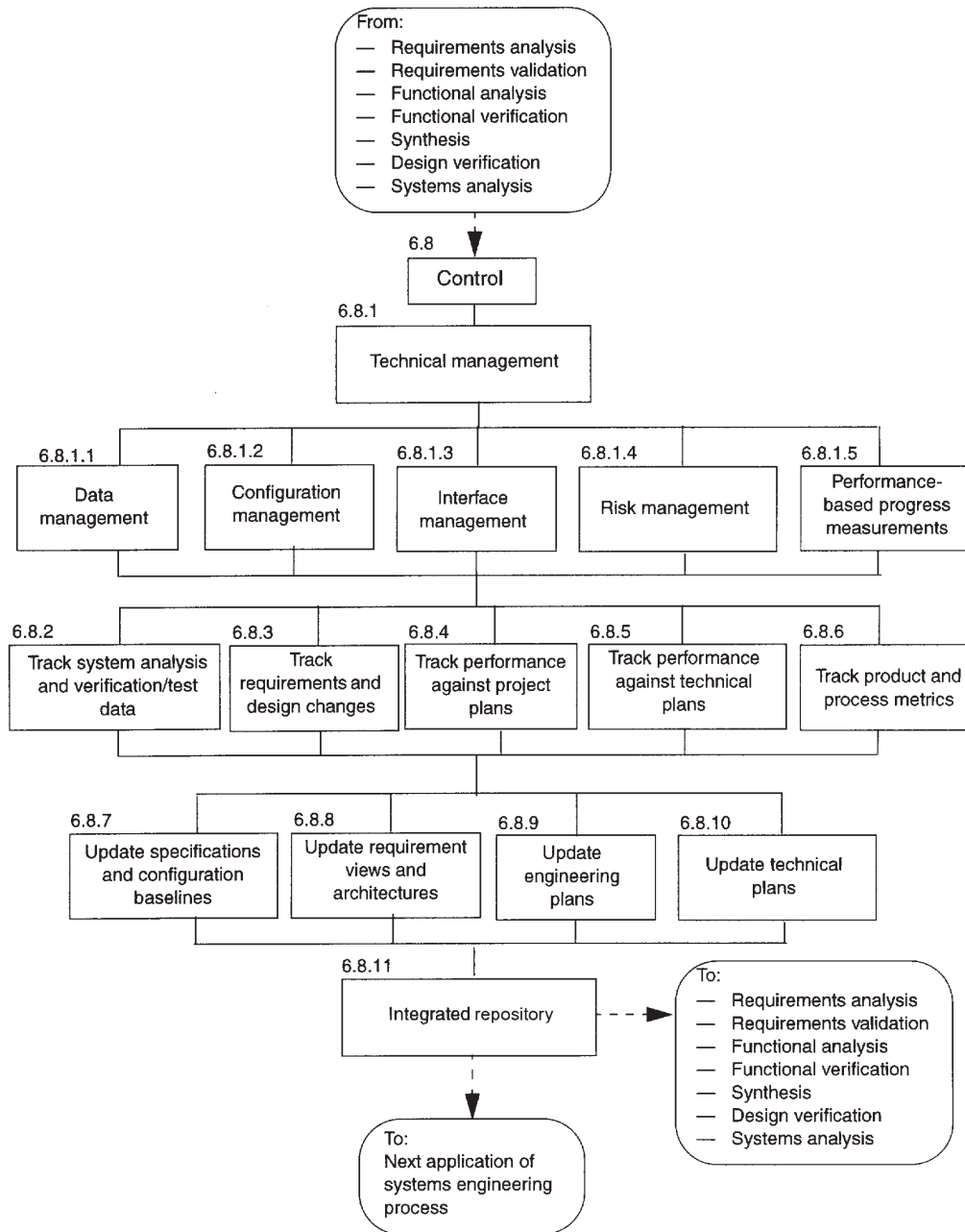
Figure 17—Control process
