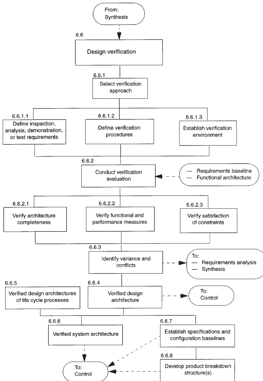
Figure 15—Design verification
