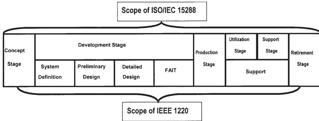
Figure C.5—Scope comparison across typical system life cycle stages
