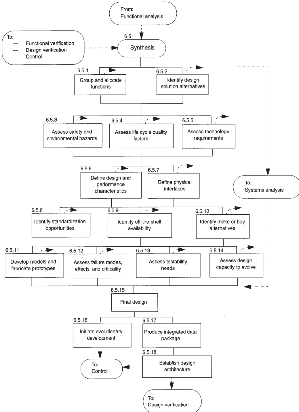
Figure 14—Synthesis process
