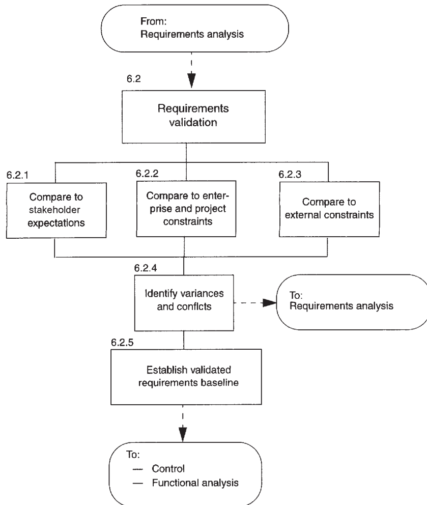
Figure 11—Requirements validation
