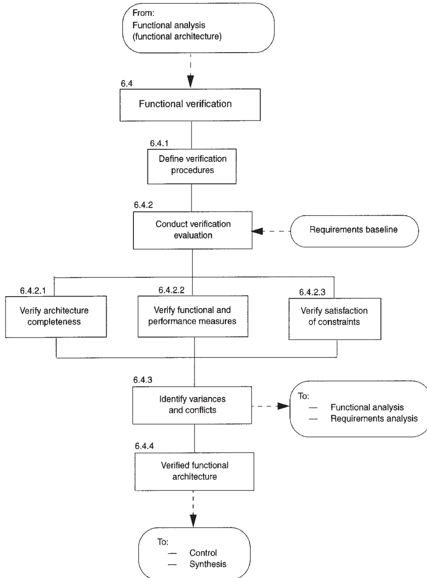
Figure 13—Functional verification
