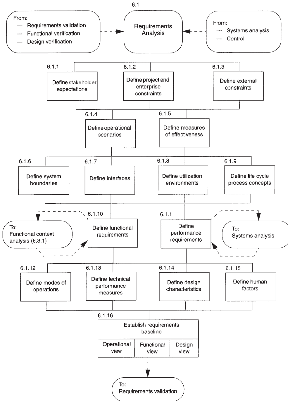
Figure 10—Requirements analysis
